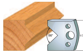
Pair of knives 690.034 Pair of limitors 691.034
