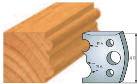
Pair of knives 690.029 Pair of limitors 691.029
