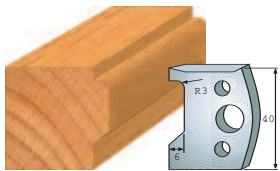
Pair of knives 690.032 Pair of limitors 691.032
