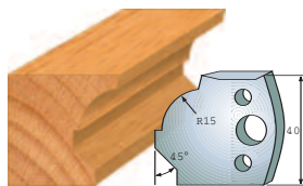
Pair of knives 690.037 Pair of limitors 691.037
