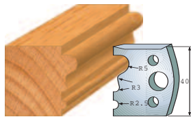
Pair of knives 690.033 Pair of limitors 691.033
