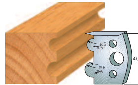
Pair of knives 690.030 Pair of limitors 691.030
