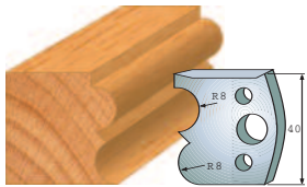
Pair of knives 690.028 Pair of limitors 691.028
