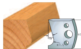
Pair of knives 690.038 Pair of limitors 691.038
