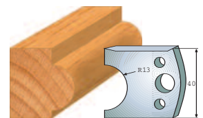
Pair of knives 690.119 Pair of limitors 691.119
