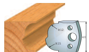
Pair of knives 690.115 Pair of limitors 691.115
