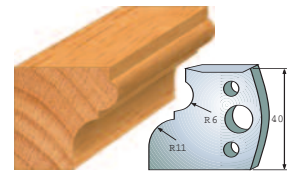
Pair of knives 690.111 Pair of limitors 691.111
