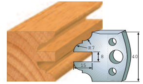
Pair of knives 690.099 Pair of limitors 691.099
