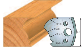
Pair of knives 690.123 Pair of limitors 691.123
