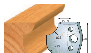
Pair of knives 690.177 Pair of limitors 691.177
