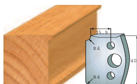
Pair of knives 690.171 Pair of limitors 691.171
