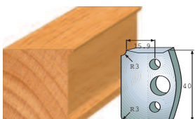
Pair of knives 690.170 Pair of limitors 691.170
