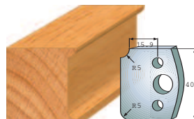
Pair of knives 690.172 Pair of limitors 691.172
