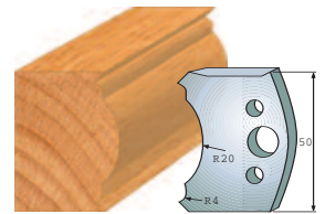
Pair of knives 690.507 Pair of limitors 691.507
