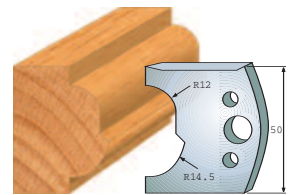
Pair of knives 690.519 Pair of limitors 691.519
