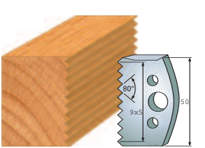
Pair of knives 690.524 Pair of limitors 691.524
